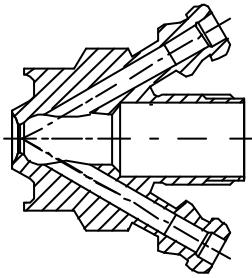
Valve body Type P Item no.: 400011
