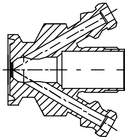
Valve body Type C Item no.: 400021
